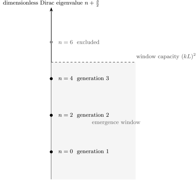
Figure 3. The emergence window. The retained sector of the RP^3 Dirac spectrum n + \frac{3}{2} ( n = 0, 2, 4, \dots ) below the window capacity (kL)^2 is the three-generation ladder. The first mode above the window, n = 6 , is excluded by the scale flow.
