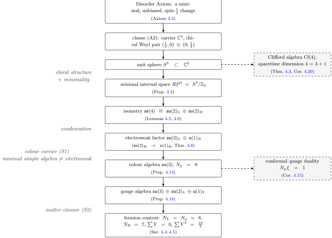
Figure 1. The emergence chain. Solid arrows carry the selections and constructions of Section 4. Dashed arrows mark derived consequences. A single minimality criterion is applied three times, to the admissible quotient (giving RP^3 ), to the symmetry group (giving SU(2) ), and to the colour algebra (giving \mathfrak{su}(3) ). The colour step is conditional on the additional colour carrier (S1) of Definition 4.11, and the fermion content is derived within the matter closure (S2) of that definition, not selected by the disorder axiom; the first two steps are selections within the disorder axiom.
